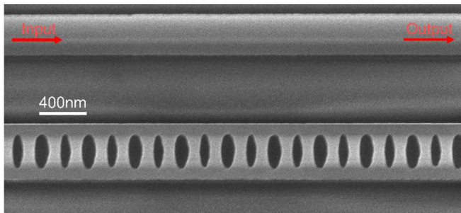
Fig. 3 SEM image of the fabricated TPC nanobeam filter.
