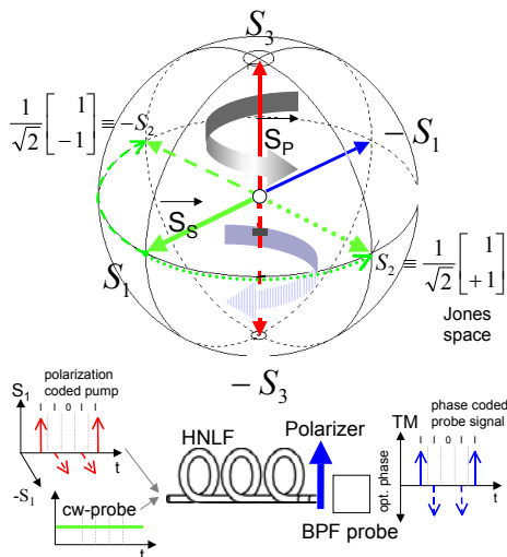
Fig. 1: Poincare sphere and Jones space representations of the NLPR.
