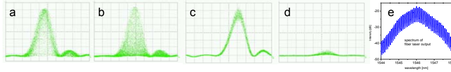
Fig.2: a) and b) interfered pulses from the fiber laser at the MZI constructive and destructive ports, respectively, c) and d) are the corresponding pulse waveform for the converted probe signal (5ps/div). and e) pump signal spectrum (0.01nm res.).
