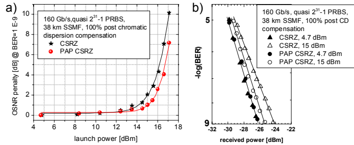
Fig.5: a) Sensitivity penalty due to NL propagation vs. launch power in SMF, b) BER curves for both formats at launch powers of 4.7 and 15 dBm in SMF.
