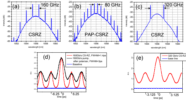
Fig. 4: spectra of a) 160-Gb/s CSRZ, b) 160-Gb/s PAP-CSRZ, c) 320-Gb/s CSRZ, and autocorrelation traces of d) 160-Gb/s and e) 320-Gb/s signals.
